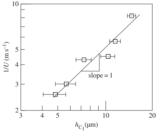
Figure 5. Correcting the linear stability prediction by accounting for the azimuthal curvature of the film in the capillary stress term of (5.2) is seen to improve the prediction of the onset of fluid instability in region (ii) of figure 4a.
